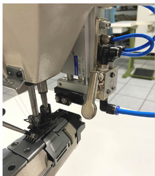
CUTTING DEVICE 164-15
