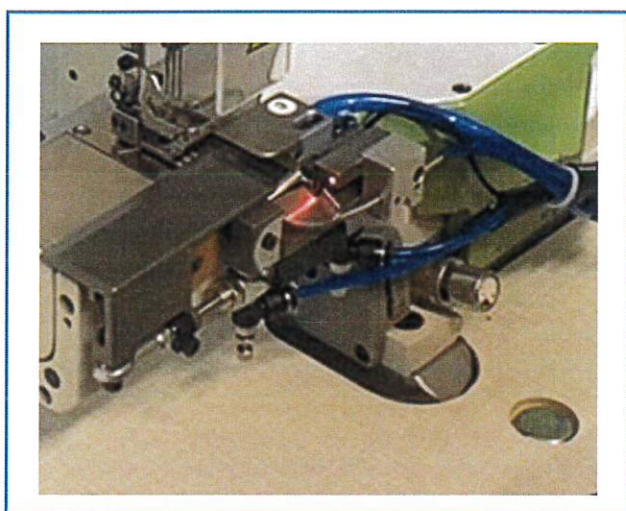
GUIDA MOBILE/SLIDING GUIDE
