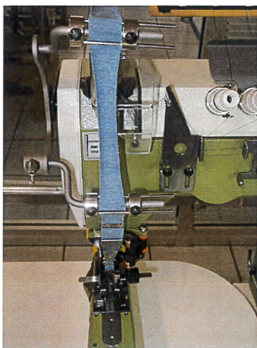
Tape rack, folder and foot
