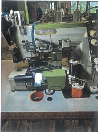
CF 3111 COMPLETE UNIT FOR SHIRT BOTTOM HEMMING OPERATION
