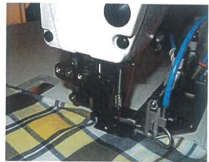
CF 3111 COMPLETE UNIT FOR SHIRT BOTTOM HEMMING OPERATION
